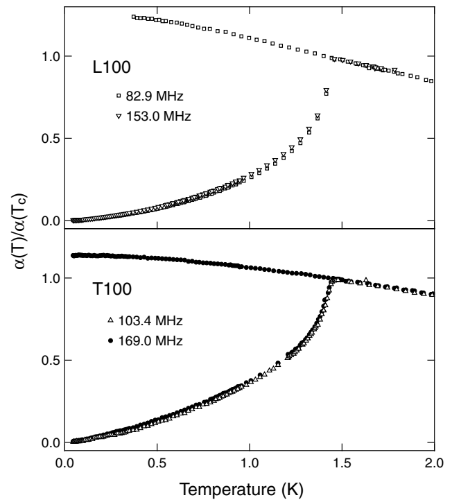
FIG. 1. Ultrasound attenuation \alpha(T) normalized at T_c , both in the superconducting state ( B = 0 ) and in the normal state ( B = 1.5\text{ T} \perp c ). We show both T100 and L100 at different frequencies to demonstrate that the shape of the curves does not depend on frequency.
