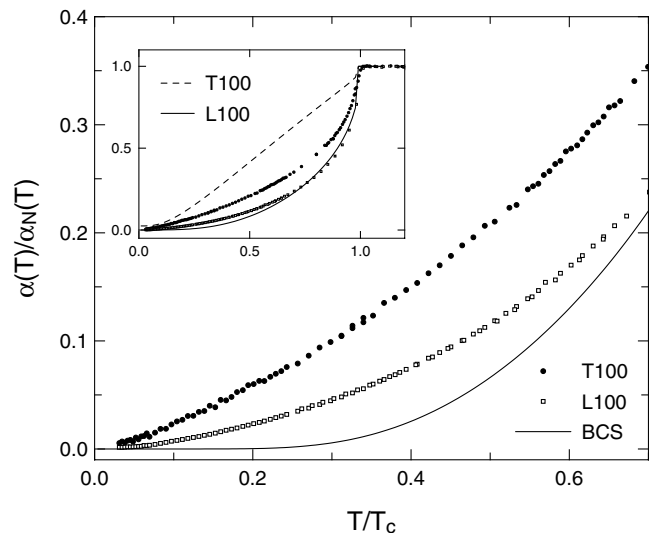
FIG. 3. \alpha(T) divided by the normal state attenuation vs reduced temperature. The solid line is the simple BCS prediction. Inset: data up to T_c , compared with calculations for f -wave discussed in the text [21].
