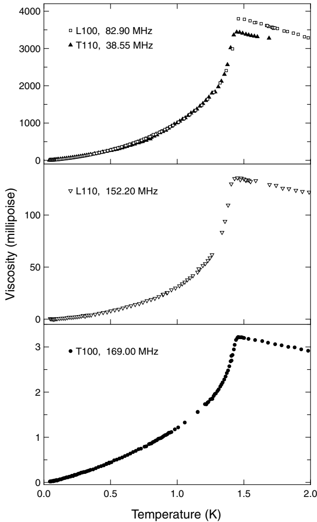
FIG. 2. Viscosity for the four in-plane modes. The viscosity \eta is related to the attenuation by \eta = \alpha \rho c_s^3 / (2\pi\nu)^2 , using a density \rho = 5.9 \text{ g/cm}^3 and the sound velocities ( c_s ) given in the text (1 poise \equiv 1 \text{ g/cm s} ). The data are extrapolated to 0 K to obtain the zero of the vertical axis.
