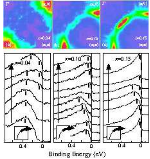
FIG. 39: Doping dependence of the MDC from experiments on NCCO with the corresponding EDC. From Ref. 86
