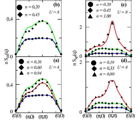
FIG. 3: Wave vector ( \mathbf{q} ) dependence of the spin and charge structure factors for different sets of parameters. Solid lines are from TPSC and symbols are our QMC data. Monte Carlo data for n = 1 and U = 8t are for 6 \times 6 clusters and T = 0.5t ; all other data are for 8 \times 8 clusters and T = 0.2t . Error bars are shown only when significant. From Ref. 37.
