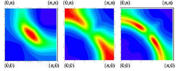
FIG. 24: MDC in the t - t' , U = 8t Hubbard model, calculated on a 4-site cluster in CDMFT. Energy resolution, \eta = 0.1t (left and middle). Left: Hole-doped dSC ( t' = -0.3t, n = 0.96 ), Middle: Electron-doped dSC ( t' = 0.3t, n = 0.93 ), Right: Same as middle with \eta = 0.02t . Note the particle-hole transformation in the electron-doped case. From Ref. 17.
