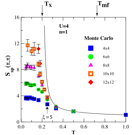
FIG. 4: Temperature dependence of S_{sp}(\pi, \pi) at half-filling n = 1 . The solid line is from TPSC and symbols are Monte Carlo data from Ref. 44. Taken from Ref. 37.
