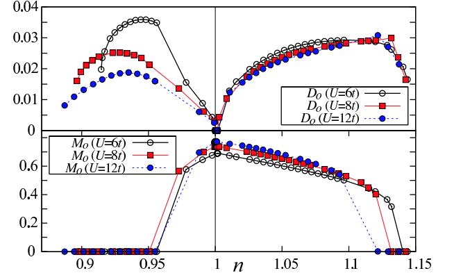
FIG. 34: Antiferromagnetic (bottom) and d -wave (top) order parameters as a function of the electron density ( n ) for t' = -0.3t , t'' = 0.2t and various values of U on a 8-site cluster, calculated in VCPT. From Ref. 19.
