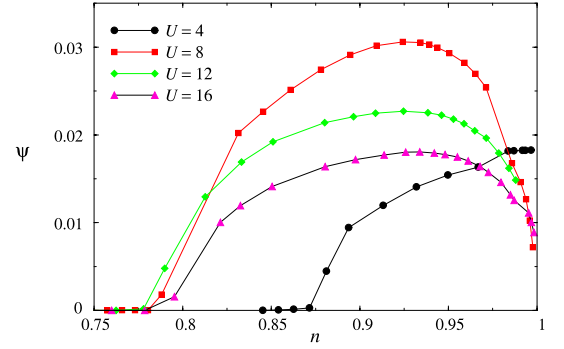
FIG. 35: d -wave order parameter as a function of n for various values of U , and t' = t'' = 0 calculated in CDMFT on a 4-site cluster. From Ref. 17.
