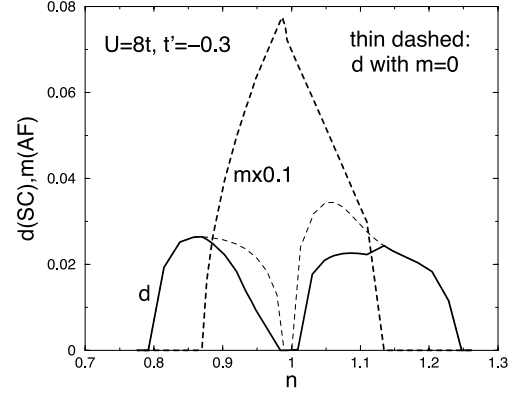
FIG. 49: Antiferromagnetic order parameter m (dashed) and d-wave (solid) order parameter obtained from CDMFT on a 2 \times 2 cluster. The result obtained by forcing m = 0 is also shown as a thin dashed line.
