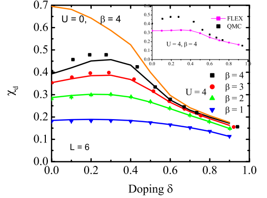
FIG. 8: Comparisons between the d_{x^2-y^2} susceptibility obtained from QMC simulations (symbols) and from the TPSC approach (lines) in the two-dimensional Hubbard model. Both calculations are for U = 4t , a 6 \times 6 lattice. QMC error bars are smaller than the symbols. Analytical results are joined by solid lines. The size dependence of the results is small at these temperatures. The U = 0 case is also shown at \beta = 4/t as the upper line. The inset compares QMC and FLEX at U = 4, \beta = 4/t . From Ref. 40.
