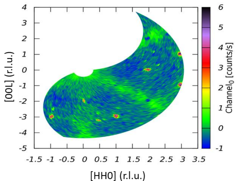
Spin Flip 60 mK
