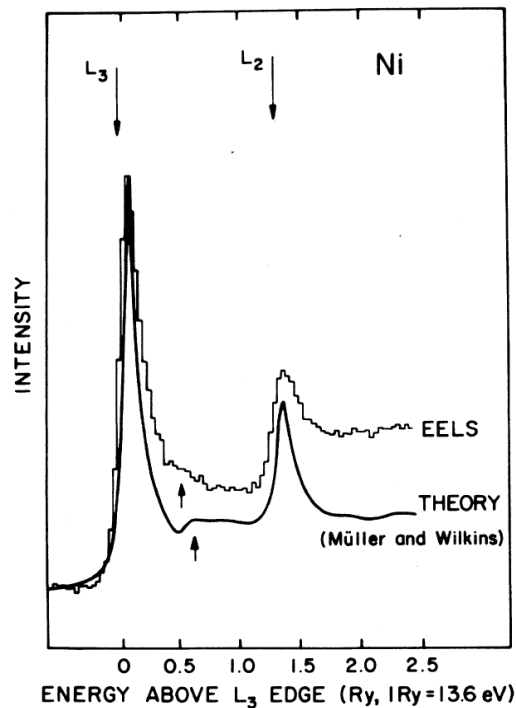
Figure 11-2 Energy loss spectroscopy for scattering from 2p_{1/2} and 2p_{3/2} states ( L_2 and L_2 ) of Nickel to empty 3d electrons that form the valence band, compared with band structure calculations. The calculations are for the Fourier transform of the density-density correlation function, as discussed in this section. That correlation function is evaluated in the dipole approximation, i.e. from the first term in the expansion of e^{-i\mathbf{q}\cdot\mathbf{r}} , because this is the leading matrix element for the atomic transition from 2p to 3d . Figure reproduced from R.D. Leapman, L.A. Grunes, and P.L. Fejes, Phys. Rev. B 26 , 614 (1982).
