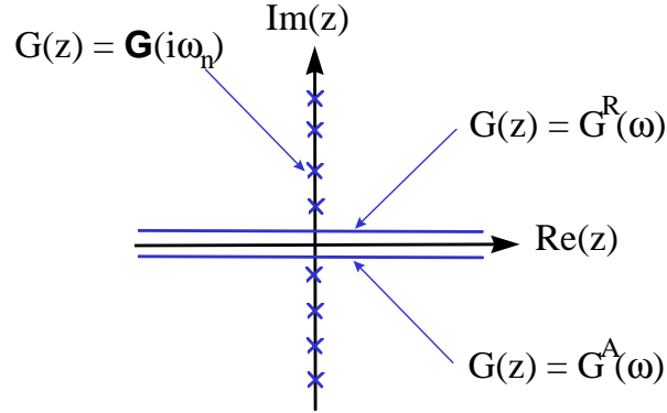
Figure 31-3 Analytical structure of G(z) in the complex frequency plane. G(z) reduces to either G^R(\omega) , G^A(\omega) or \mathcal{G}(i\omega_n) depending on the value of the complex frequency z . There is a branch cut along the real axis.
