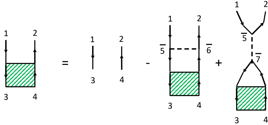
Figure 37-2 Integral equation for \delta\mathcal{G}/\delta\phi in the Hartree-Fock approximation.
