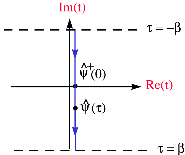
Figure 31-1 Contour for time ordering in imaginary time. Only the time difference is important. The contour is translated slightly along the real-time axis for clarity.
