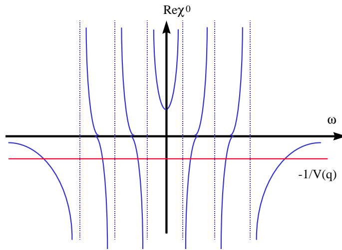
Figure 41-4 Graphical solution for the poles of the charge susceptibility in the interacting system.
