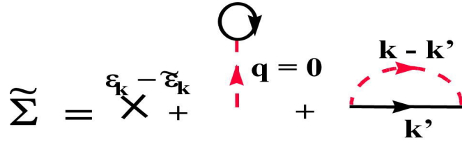
Figure 42-3 Effective medium point of view for the Hartree-Fock approximation. In this figure, the propagators are evaluated with the effective medium \tilde{H}_0 .
