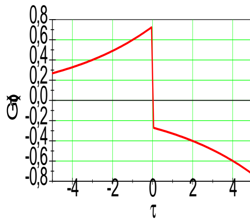
Figure 31-6 G_0(\mathbf{p}, \tau) for a value of momentum below the Fermi surface.
