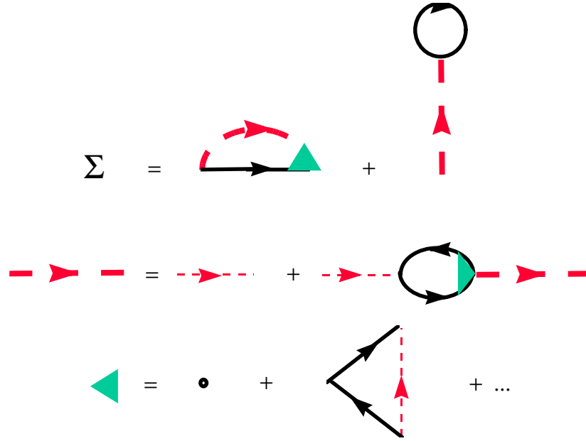
Figure 48-1 Exact resummation of the diagrammatic perturbation expansion. The dressed interaction on the second line involves the one-interaction irreducible polarisation propagator. The last line gives the first terms of the diagrammatic expansion for the vertex corrections.
