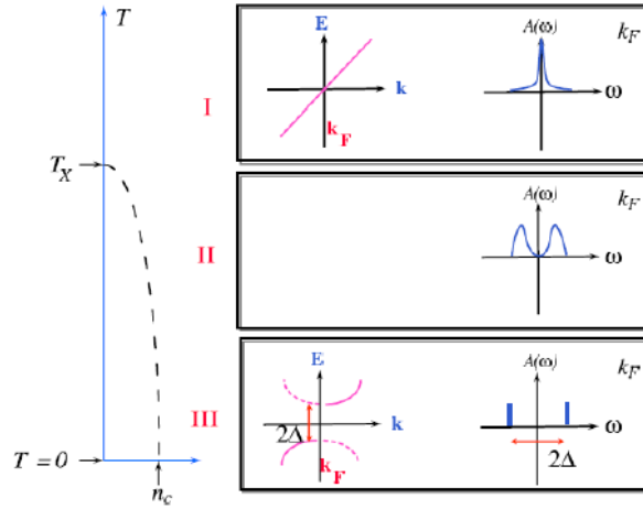
Figure 55-1 Cartoon explanation of the pseudogap due to precursors of long-range order. When the antiferromagnetic correlation length \xi becomes larger than the thermal de Broglie wavelength, there appears precursors of the T = 0 Bogoliubov quasi-particles for the long-range ordered antiferromagnet. This can occur only in the renormalized classical regime, below the dashed line on the left of the figure.
