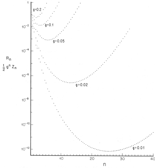
Figure 47-1 Asymptotic expansion of Z(g) for different values of g . The residual error R_n 's plotted for the half-integer values. From J.W. Negele and H. Orland, op. cit. p.56
