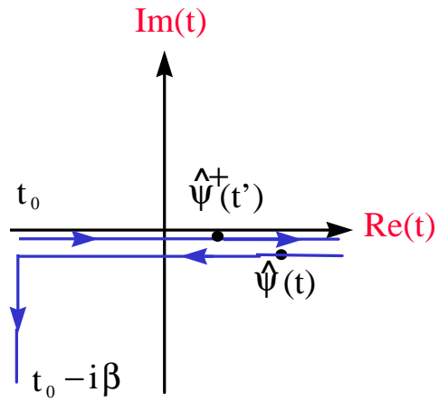
Figure 30-2 Keldysh-Schwinger contour.
