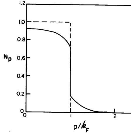
Figure 45-5 Momentum density in the RPA approximation for an electron gas with r_s = 3.97 . From E. Daniel and S.H. Vosko, Phys. Rev. 120 , 2041 (1960).
