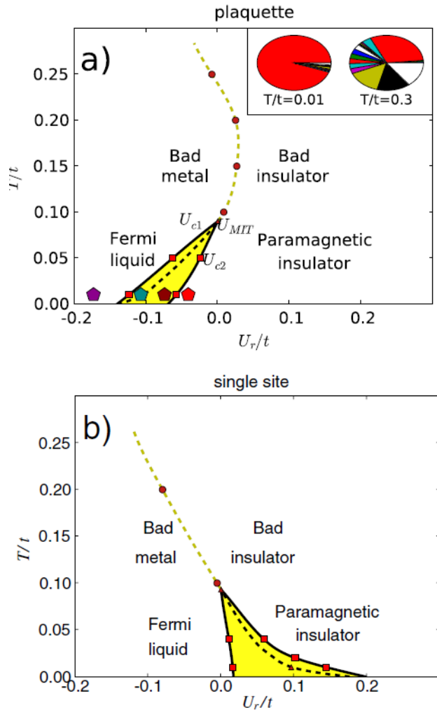
Figure 56-1 First order transition for the Mott transition. (a) shows the result for two dimensions obtained for a 2 \times 2 plaquette in a bath. In (b), the result obtained for a single site. The horizontal axis is U_r = (U - U_{MIT})/U_{MIT} with U_{MIT} = 6.05t in the plaquette case and U = 9.35t in the single site case.
