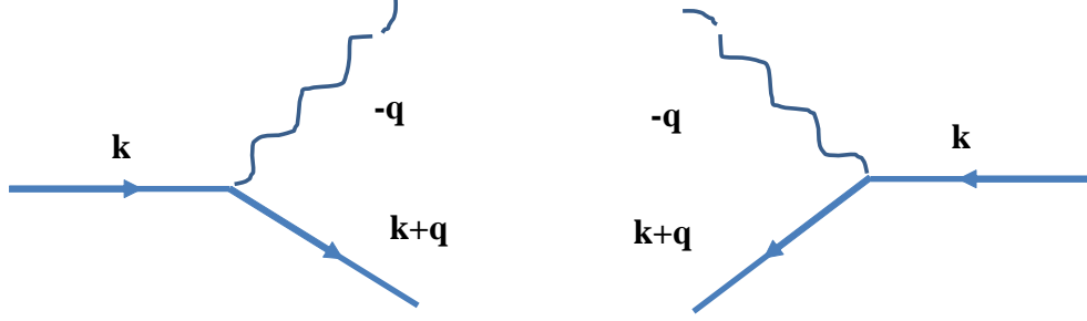
Figure 45-3 Schematic representation of the processes contained in the imaginary part of the self-energy. On the left, an electron in with momentum and frequency \mathbf{k}, \omega decays into another a quasiparticle \mathbf{k} + \mathbf{q}, \zeta_{\mathbf{k}+\mathbf{q}} plus a particle-hole excitation -\mathbf{q}, \omega - \zeta_{\mathbf{k}+\mathbf{q}} that can be a plasmon, depending on the conditions on wave-vector and frequency. On the right, the analogous process for a hole.
