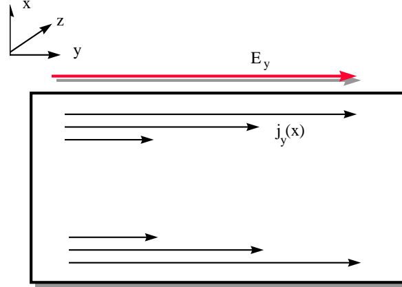
Figure 15-1 Application of a transverse electric field: skin effect.
