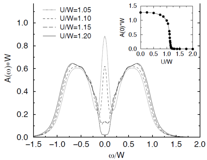
Figure 56-2 decrease for U 1:1 W; from Ref. [78] in Vollhardt in Mancini.
