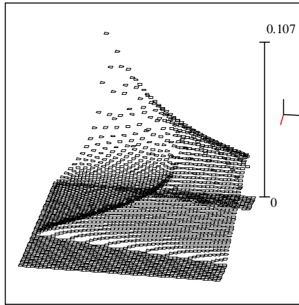
Figure 39-3 Imaginary part of the Lindhard function in d = 2 . Axes like in the d = 1 case.
