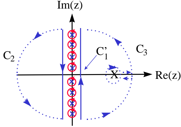
Figure 31-7 Evaluation of fermionic Matsubara frequency sums in the complex plane.
