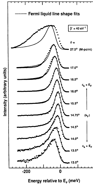
Figure 32-1 ARPES spectrum of 1 - T - TiTe_2 , after R. Claessen, R.O. Anderson, J.W. Allen, C.G. Olson, C. Janowitz, W.P. Ellis, S. Harm, M. Kalning, R. Manzke, and M. Skibowski, Phys. Rev. Lett 69 , 808 (1992).
