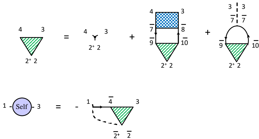
Figure 49-2 \delta\mathcal{G}/\delta\phi has been separated in two parts: the last term of the top line that comes from \delta\Sigma/\delta\mathcal{G} of the Hartree term in \Sigma and the blue box that represents the rest. That blue box appears both on the top and the bottom line. The top line is the same figure as the preceding one, but with the two external legs amputated. Comparing with the equation for the self-energy in the previous figure, we see that the self-energy can now be written entirely in terms of the green triangle, also known as fully reducible vertex.
