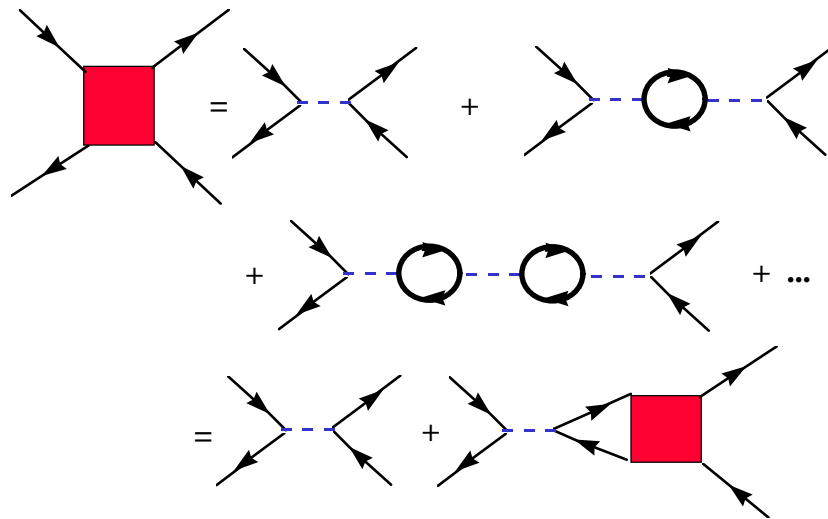
Figure 24-4 Bubble diagrams for particle-hole excitations.
