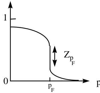
Figure 32-4 Qualitative sketch of the zero-temperature momentum distribution in an interacting system.
