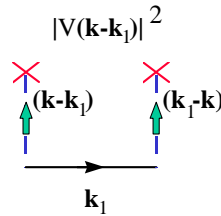
Figure 21-6 Second order irreducible self-energy (before impurity averaging). Note that \mathbf{k}_1 \neq \mathbf{k} . That is why this diagram is irreducible.
